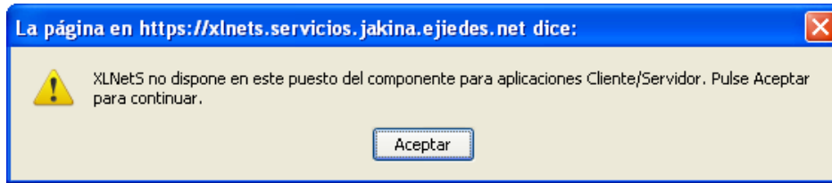
Figura 9: Aviso XLNets
